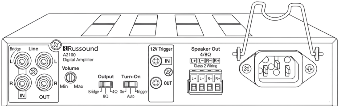
REAR VIEW OF AMPLIFIER
