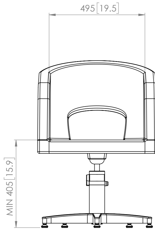
PICTURED WITH 125 HYDRAULIC & CAPITAL BASE
