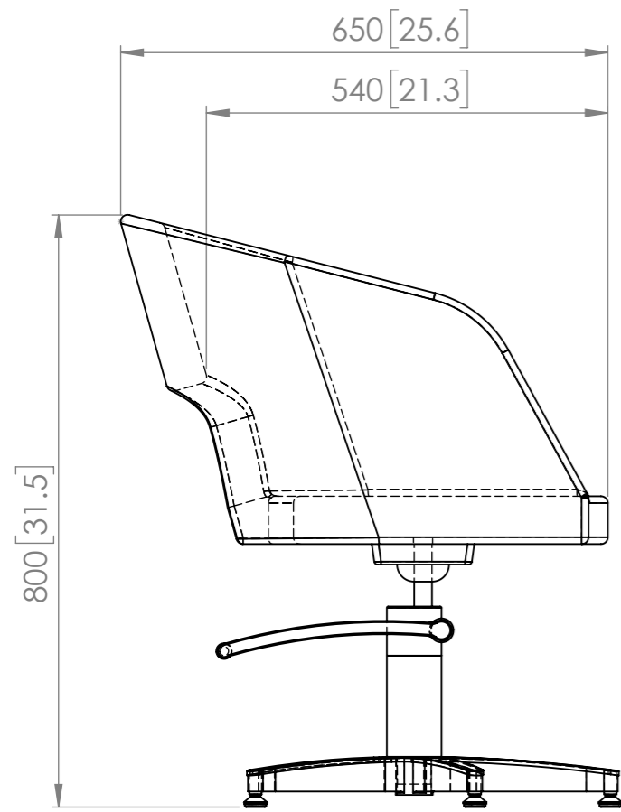
PICTURED WITH 125 HYDRAULIC & CAPITAL BASE
